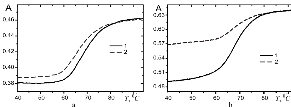
Fig. 3. Thermal denaturation (1) and renaturation (2) profiles for bi-Pt/DNA (a) and cis-DDP/DNA (b) complexes ( r = 0.03 ).
