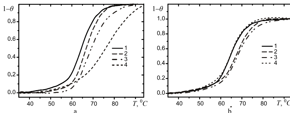
Fig. 2. Melting curves of bi-Pt/DNA (a) and cis-DDP/DNA (b) complexes in 10^{-3} M NaCl + 10^{-2} M NaClO 4 solution: r = 0 (1); 0.0003 (2); 0.03 (3); 0.3 (4).
