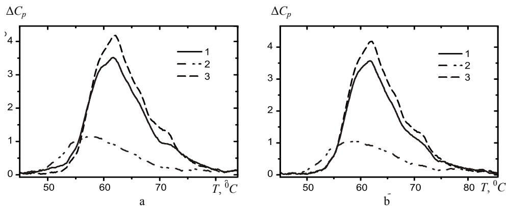
Fig. 4. Microcalorimetric melting (1) and double melting (2) curves of bi-Pt/DNA (a) and cis-DDP/DNA (b) complexes ( r = 0.03 ) and the melting curve of pure DNA (3).
